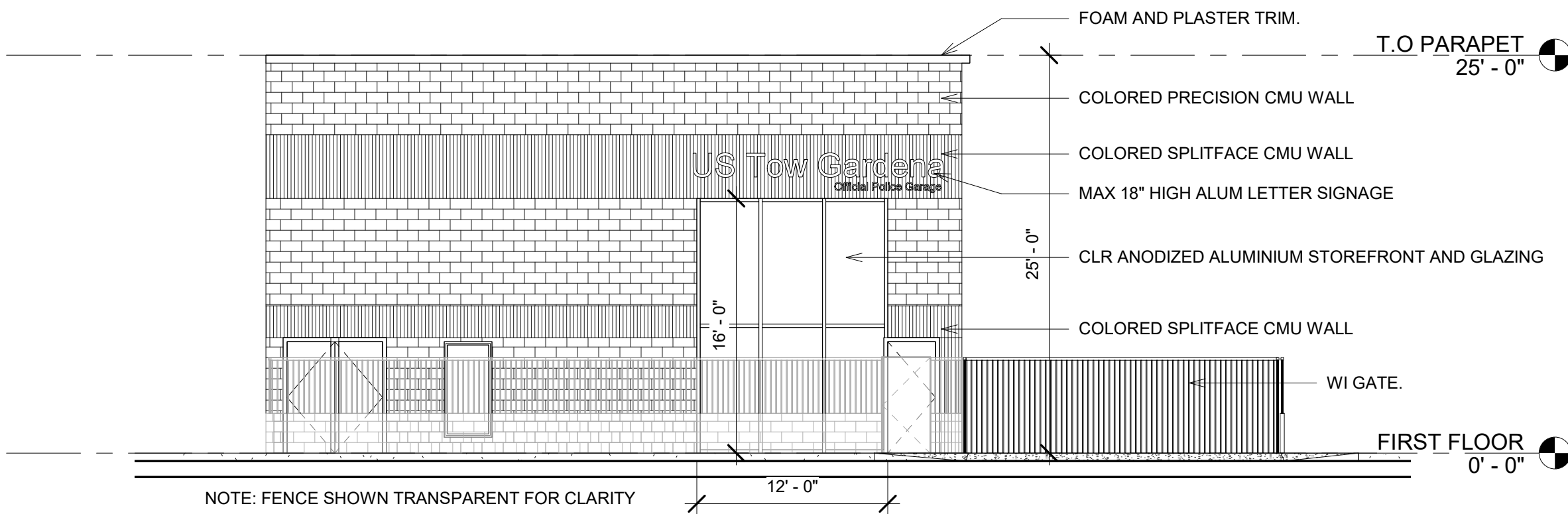
1 NORTH ELEVATION
