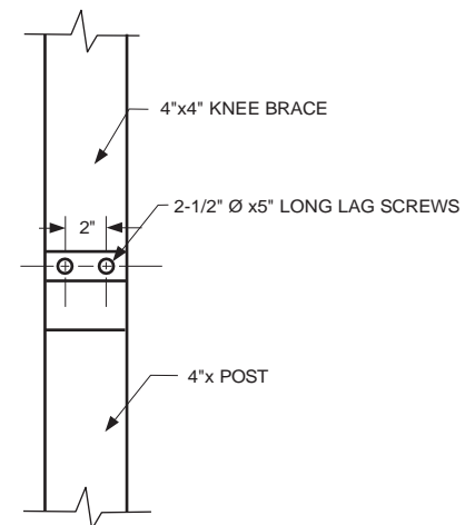
DETAIL "E"
