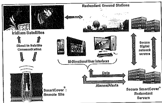
SmartCover® communications system architecture
